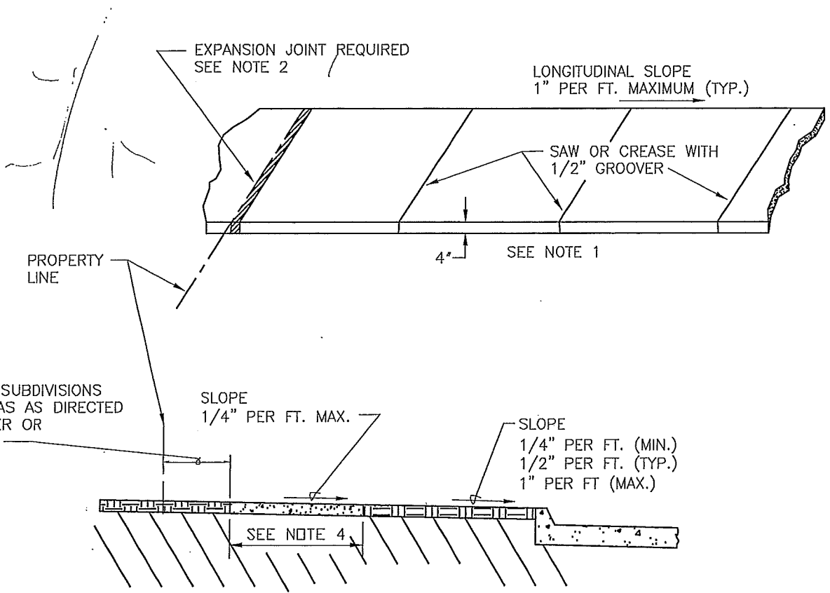
TYPICAL CROSS SECTION TYPICAL SIDEWALK
